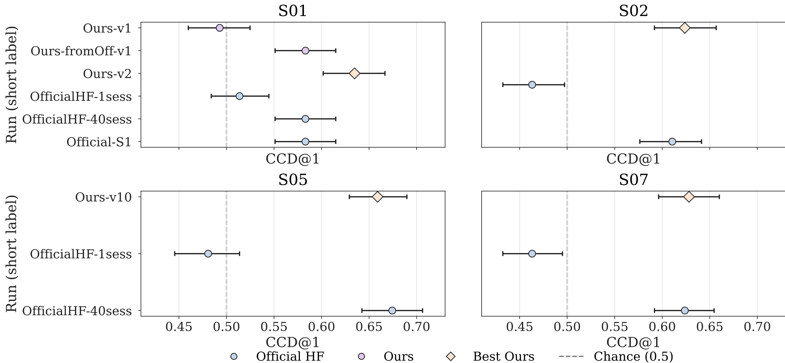
CCD@1 on shared982 (pooled, hardneg, K=1)
