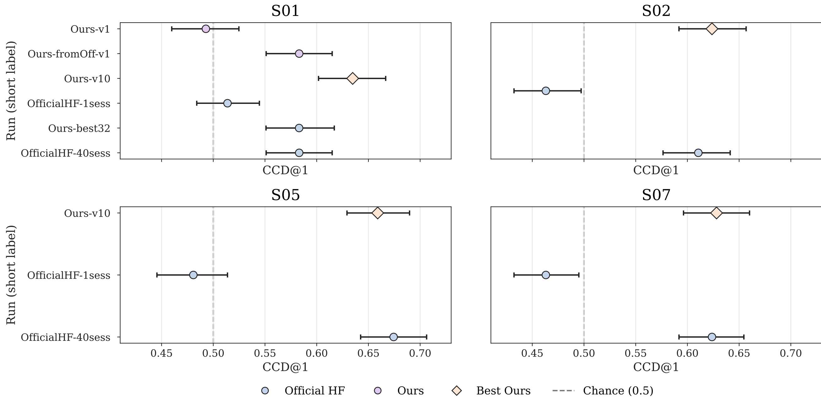
CCD@1 on shared982 (pooled, hardneg, K=1)
