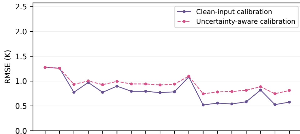
Grouping / TD-Clear
