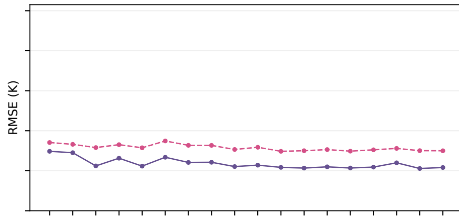
Parameterization / TD-Clear
