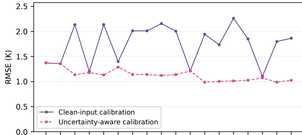
Grouping / TD-All
