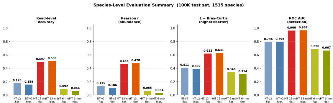
Figure 4.11: Species-level evaluation summary across six models (100K independent test set, 1,535 species). From left: read-level accuracy, Pearson r , 1 – Bray-Curtis (higher is better), and ROC AUC for binary species detection. The MT 13-mer models cross the practical utility threshold at ~50% read accuracy; all 6-mer-based models fall below the threshold regardless of backbone or hierarchical masking.
