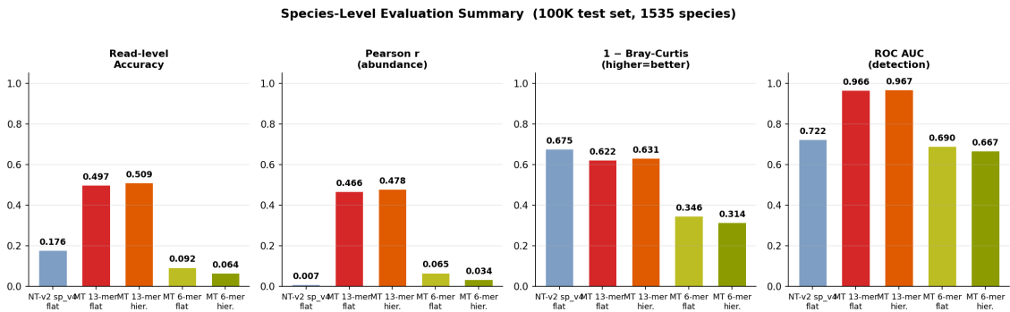
Figure 4.11: Species-level evaluation summary across five models (100K independent test set, 1,535 species). From left: read-level accuracy, Pearson r , 1 - Bray-Curtis (higher is better), and ROC AUC for binary species detection. The MT 13-mer models cross the practical utility threshold at ~50% read accuracy; all 6-mer-based models fall below the threshold regardless of backbone or hierarchical masking.
