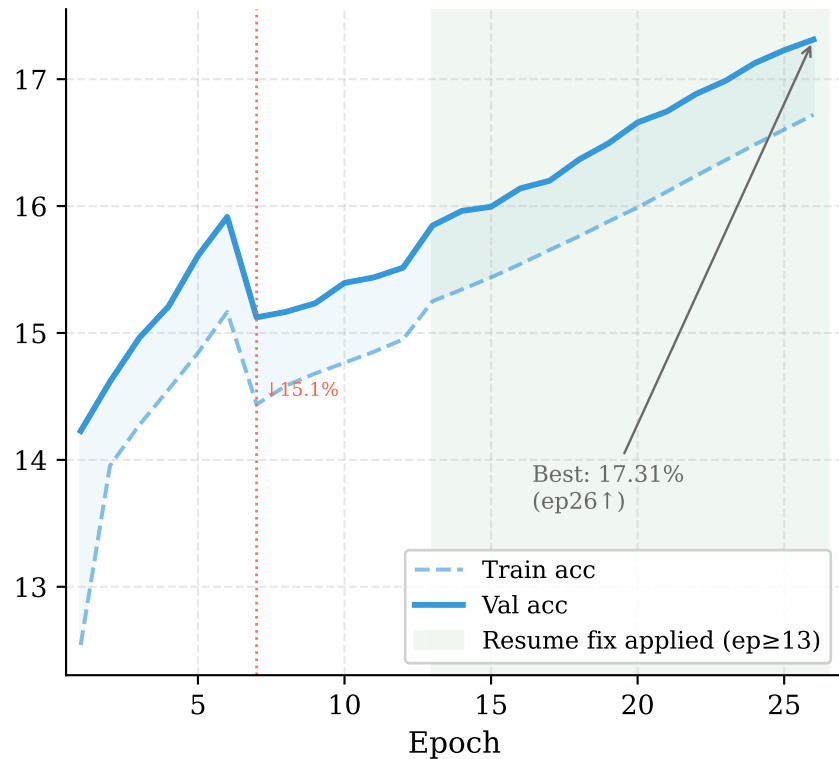
sp\_v4 — Species (1,535 classes, 50M reads)
