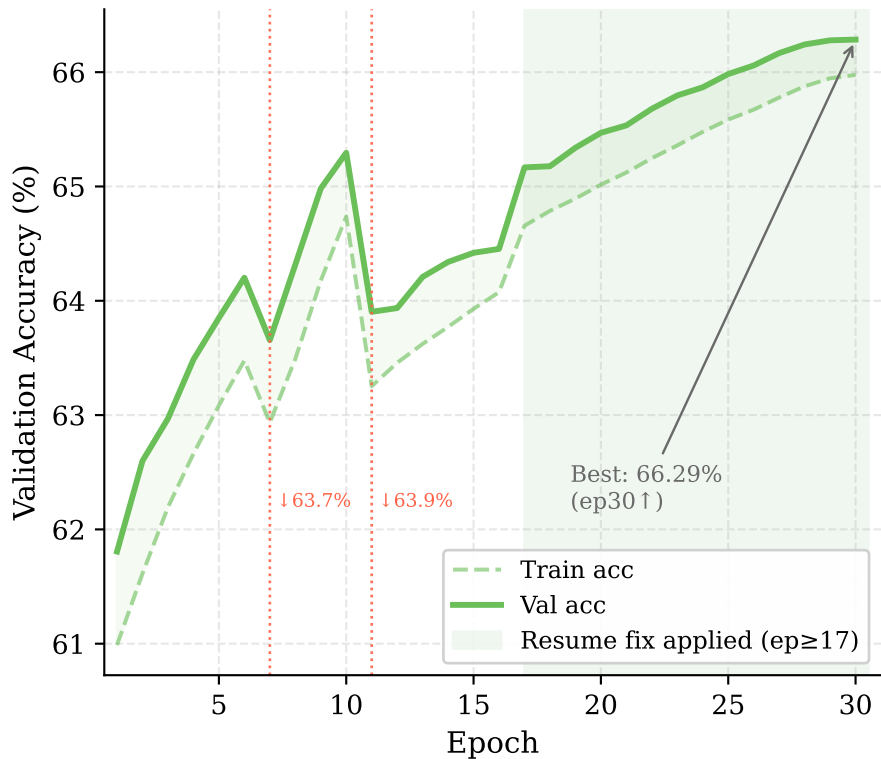
v9 — Genus (120 classes, 50M reads)
