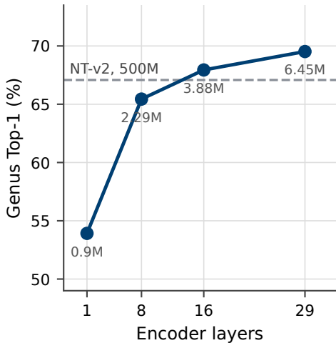
(b) Depth alone: +15.60 pp
