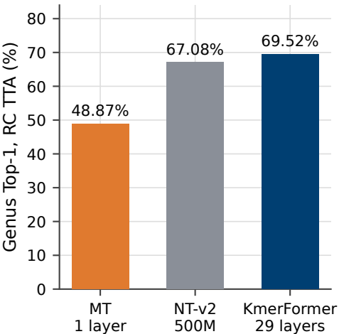
(a) At a shared 6-mer tokenizer
