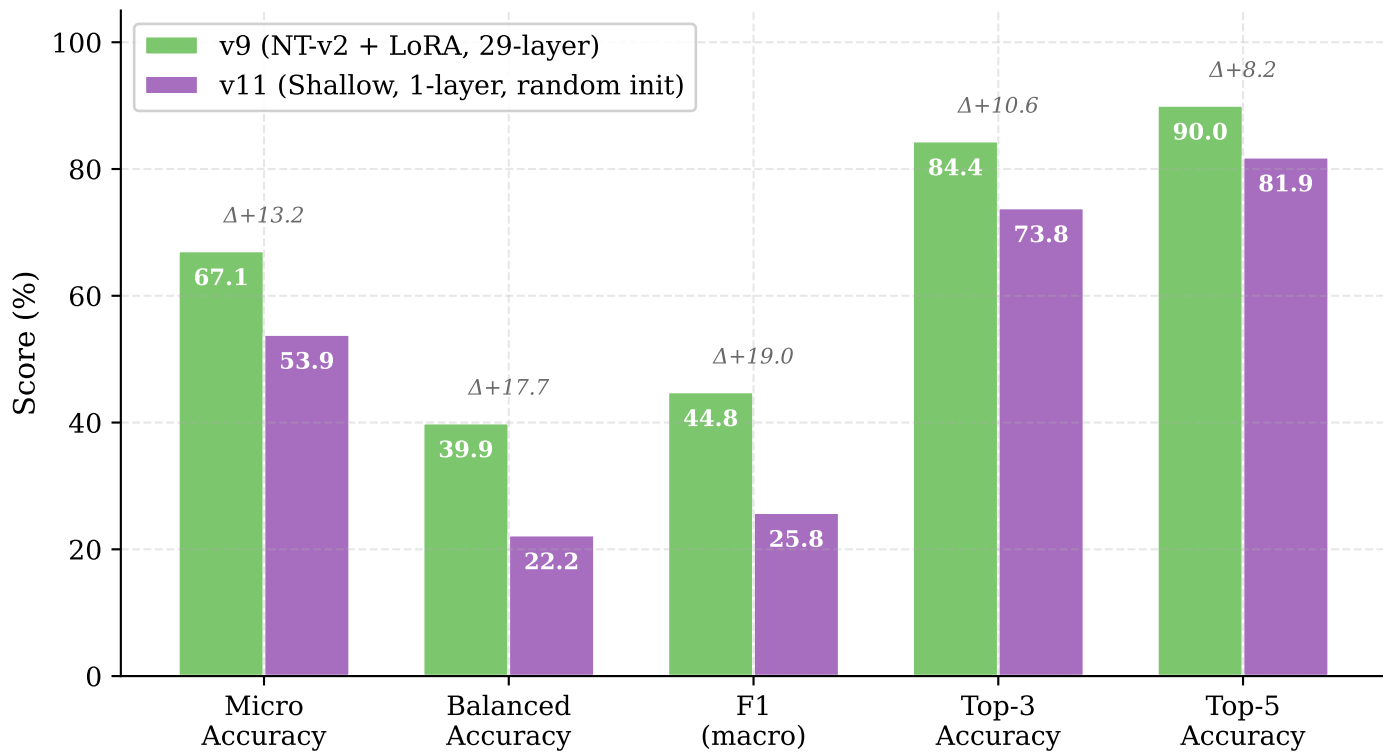
Backbone Ablation: Pre-trained NT-v2 vs. Shallow Transformer (50M balanced reads)
