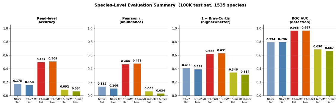
Figure 4.11: Species-level evaluation summary across six models (100K independent test set, 1,535 species). From left: read-level accuracy, Pearson r , 1 - Bray-Curtis (higher is better), and ROC AUC for binary species detection. The MT 13-mer models cross the practical utility threshold at \sim 50\% read accuracy; all 6-mer-based models fall below the threshold regardless of backbone or hierarchical masking.
