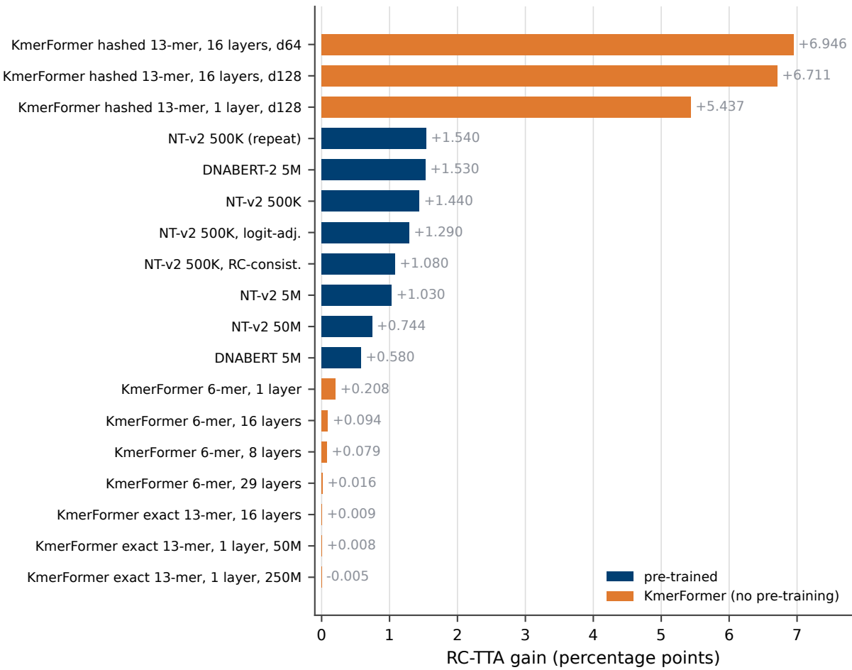
RC-TTA gains depend on tokenizer and configuration
