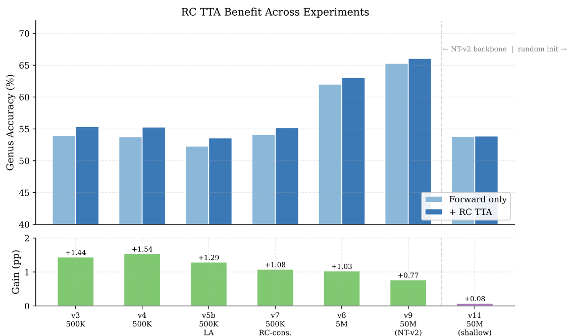
Figure 4.4: RC TTA benefit across experiments. Top: forward-only vs. RC TTA accuracy. Bottom: absolute gain in percentage points. RC TTA provides a consistent +1.0–+1.5 pp for pre-trained models (left group) and +0.08 pp for the randomly initialized shallow Transformer (v11, right group), supporting the interpretation that RC TTA corrects pre-training-induced strand biases rather than stochastic inference noise.
