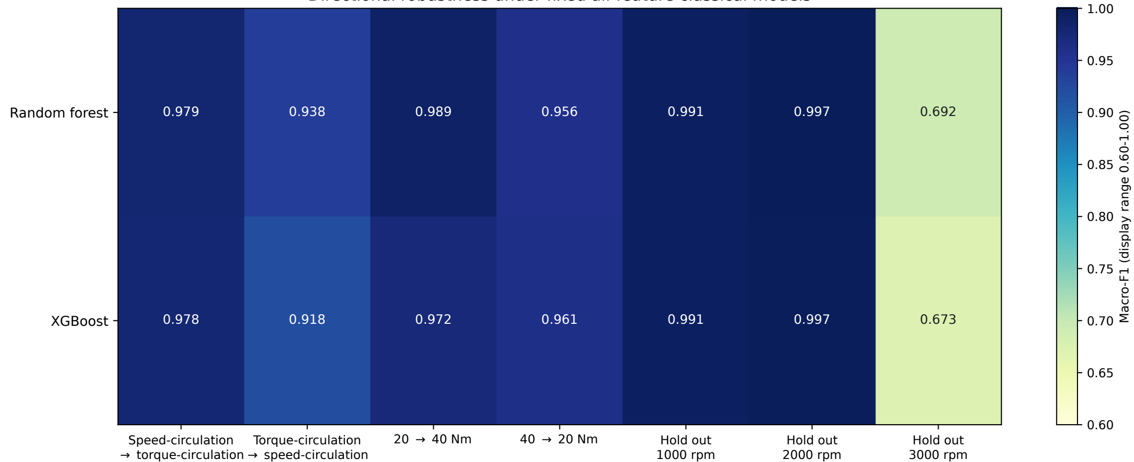
Directional robustness under fixed all-feature classical models
