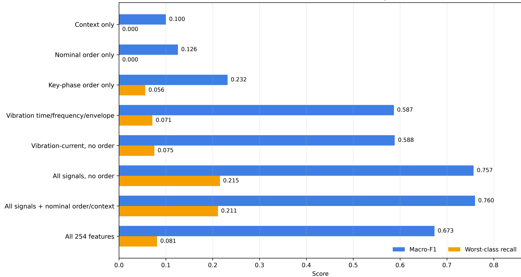
Exact feature-block evidence for the 3000-rpm holdout
