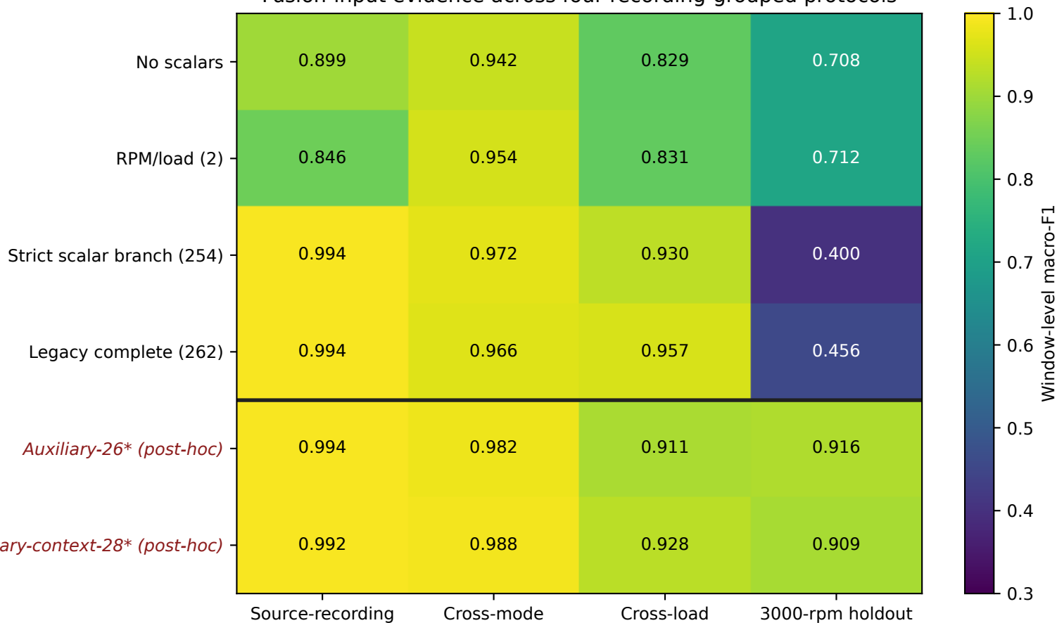
Fusion-input evidence across four recording-grouped protocols
