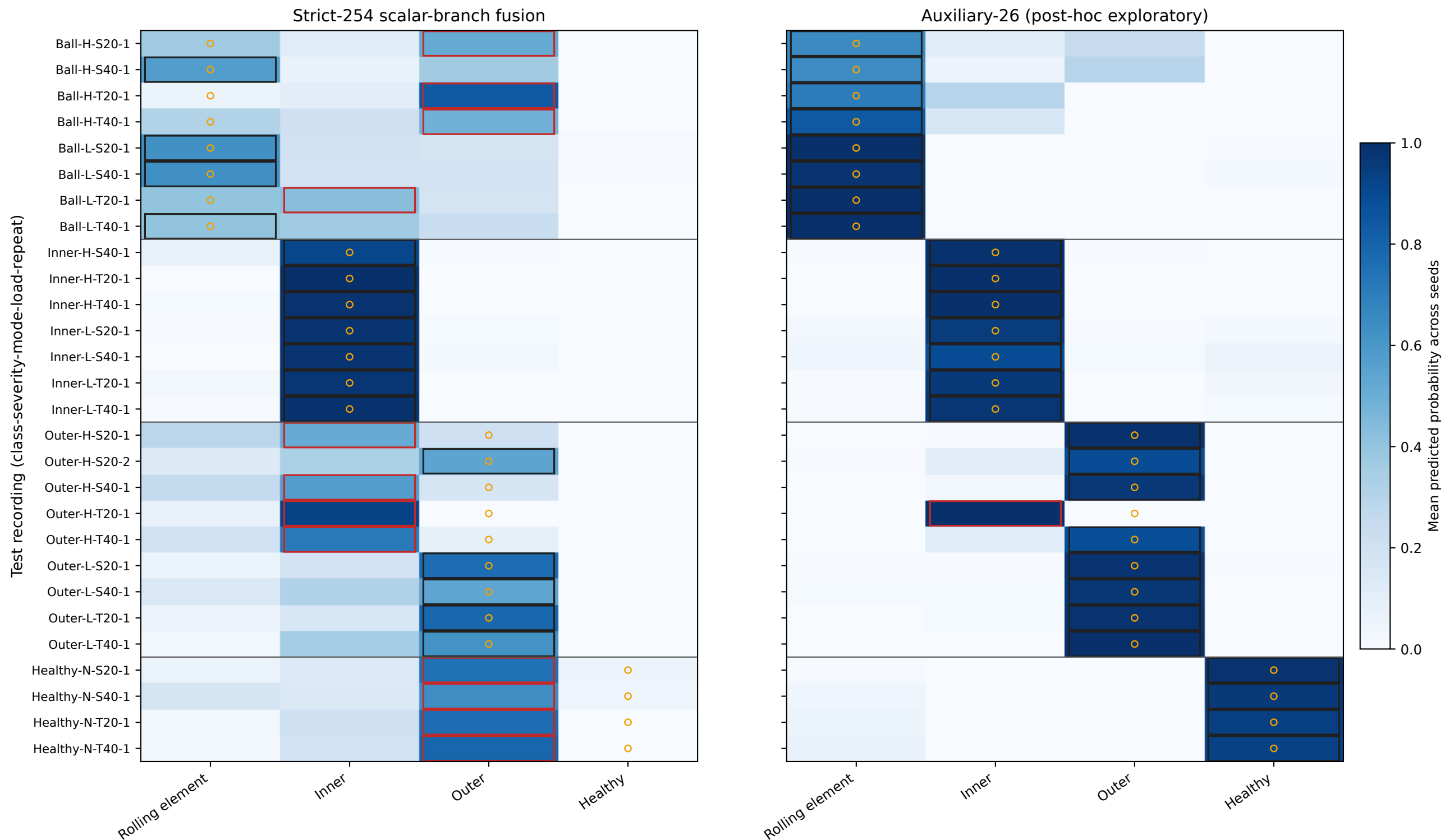
Per-recording probability audit on the 3000-rpm holdout Boxes mark predicted classes (red = error); orange circles mark true classes
