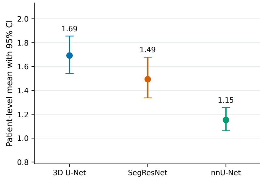
ASSD, finite values (mm; lower is better)
