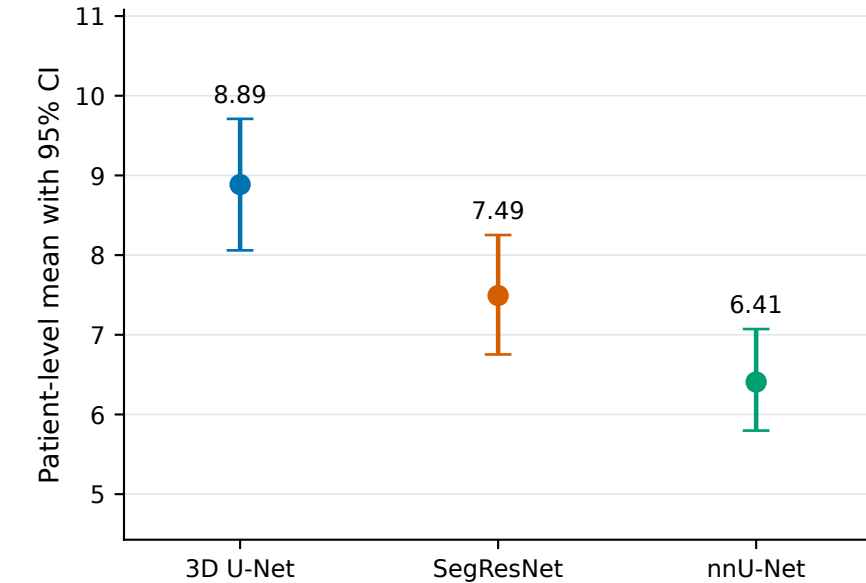
HD95, finite values (mm; lower is better)
