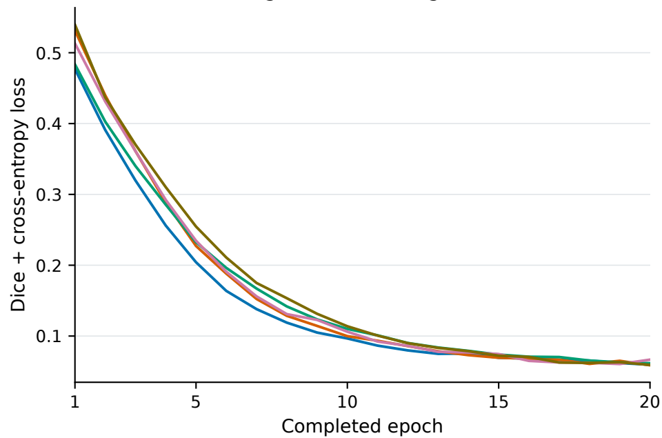
SegResNet: training loss
