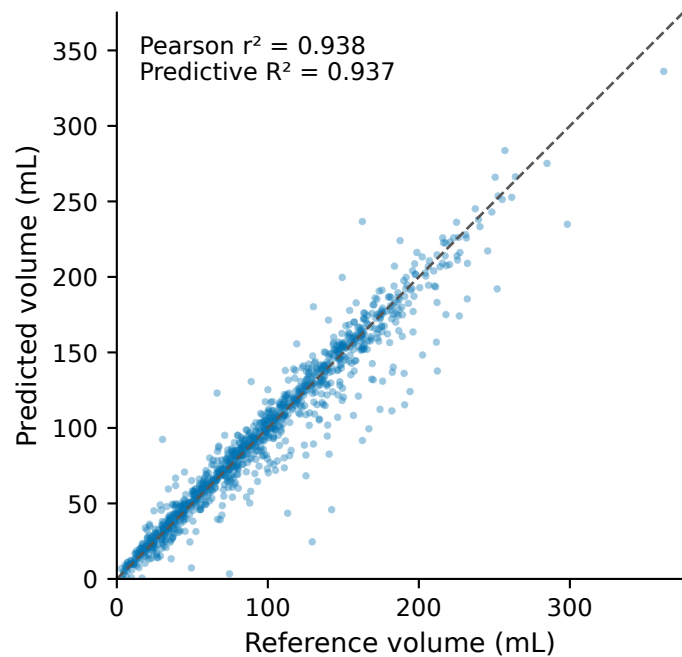
3D U-Net
