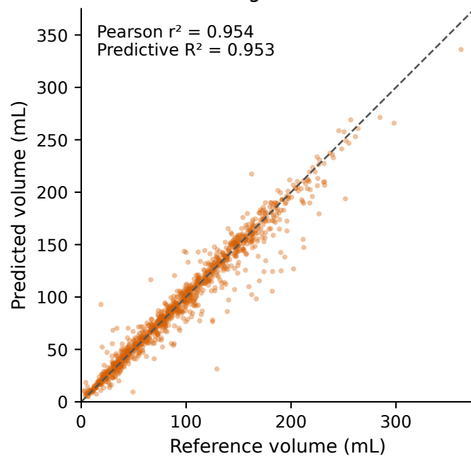
SegResNet
