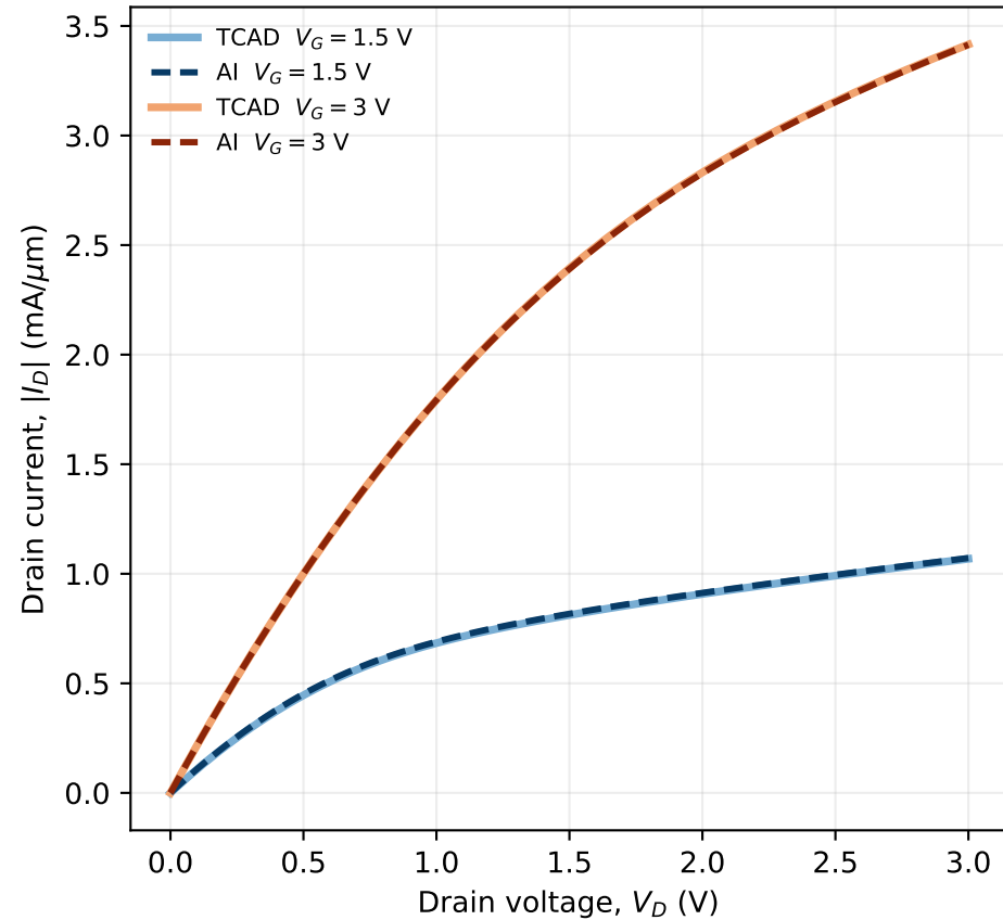
(a) Output characteristics
