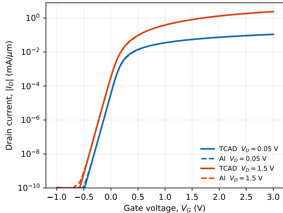
(b) Transfer characteristics
