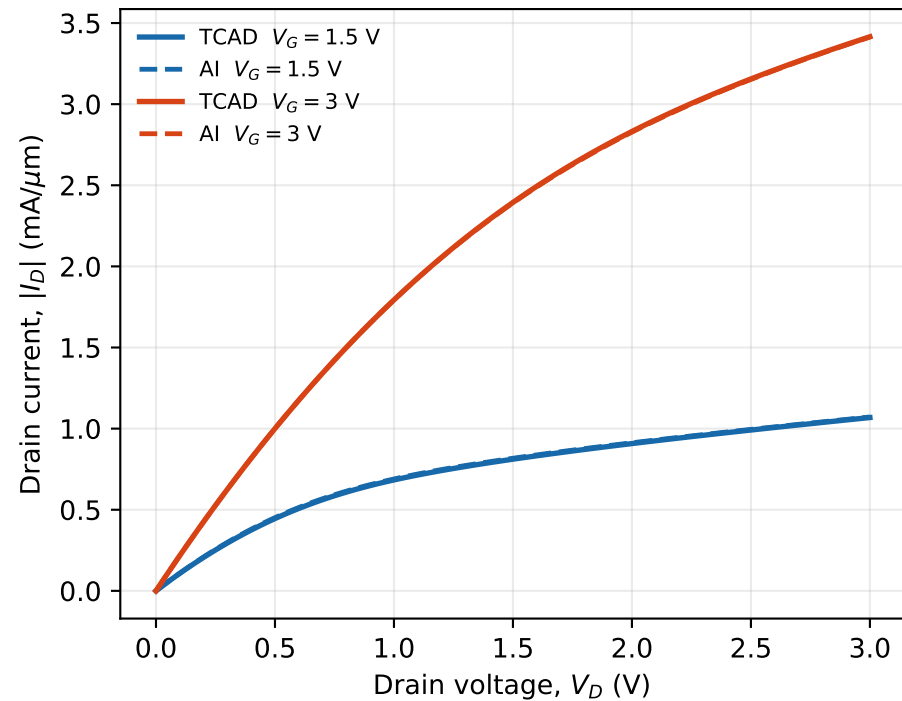
(a) Output characteristics
