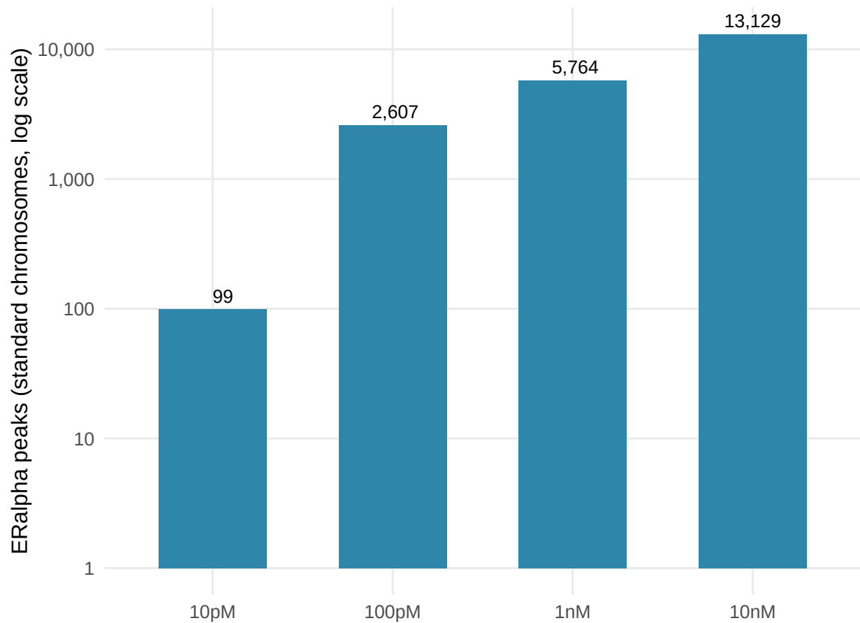
Dose-response: real, verified ERalpha peak counts
