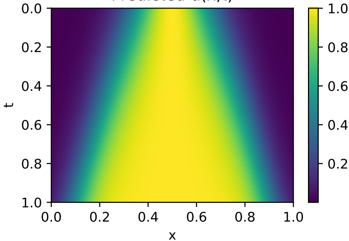
Predicted u(x,t)
