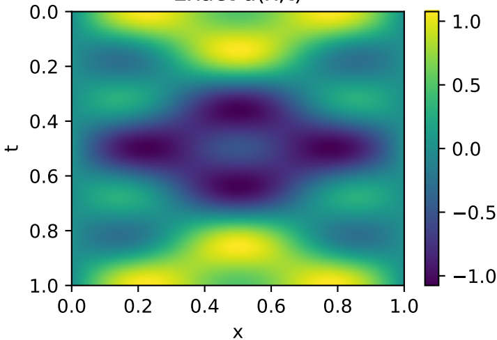
Exact u(x,t)
