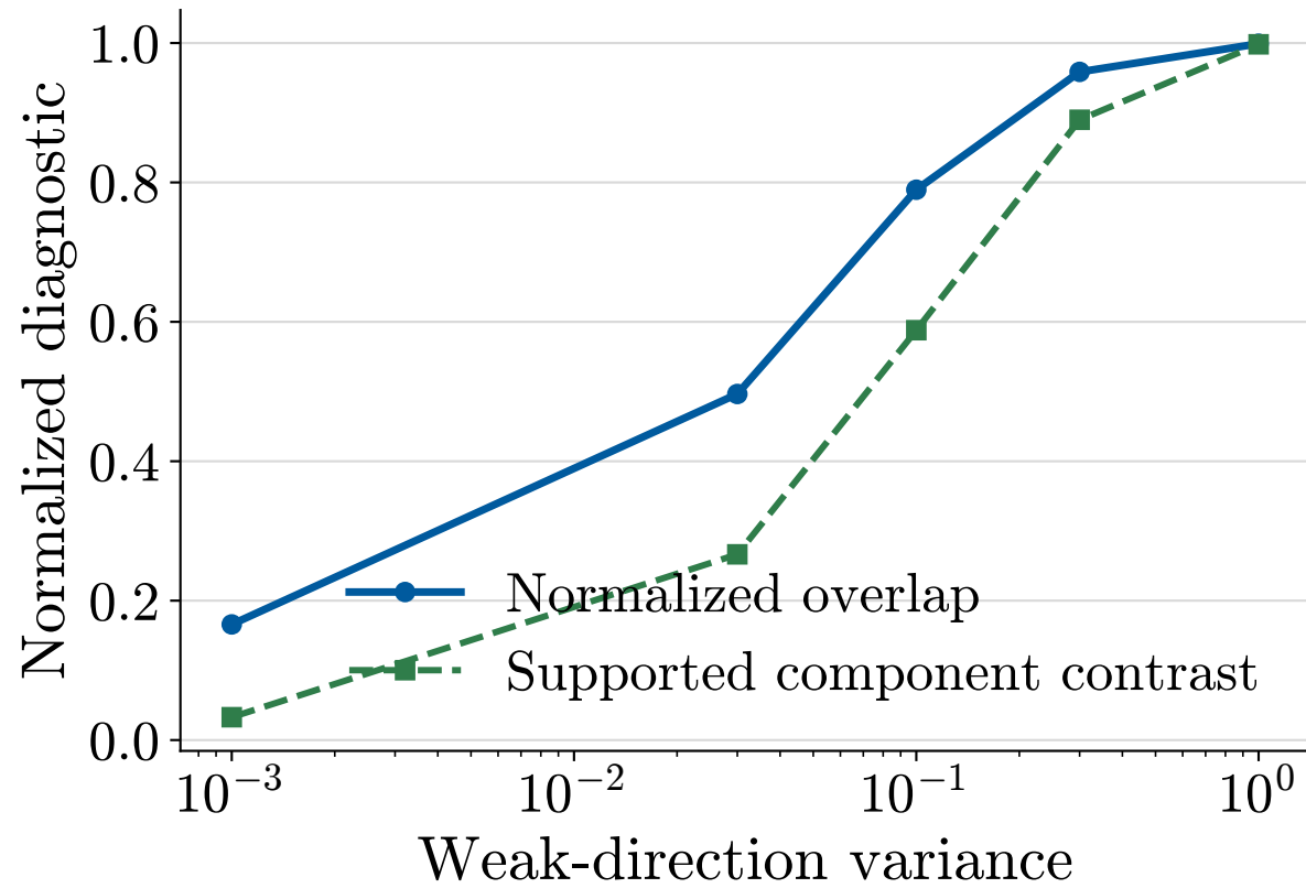
Overlap diagnostics
