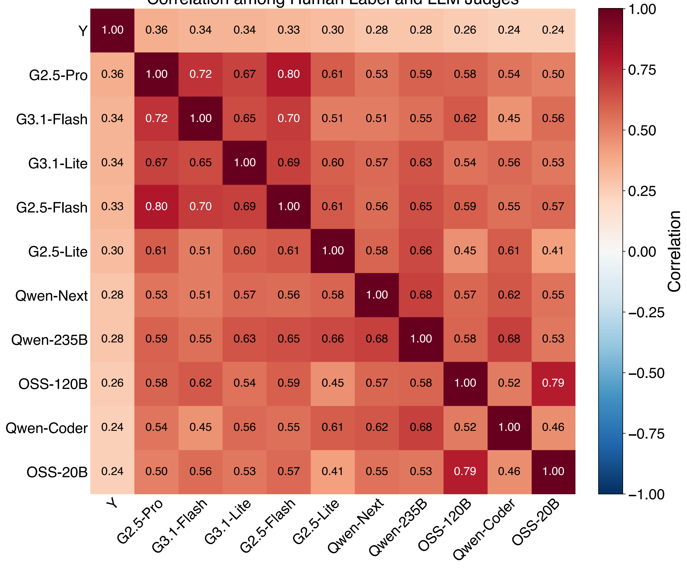
Correlation among Human Label and LLM Judges
