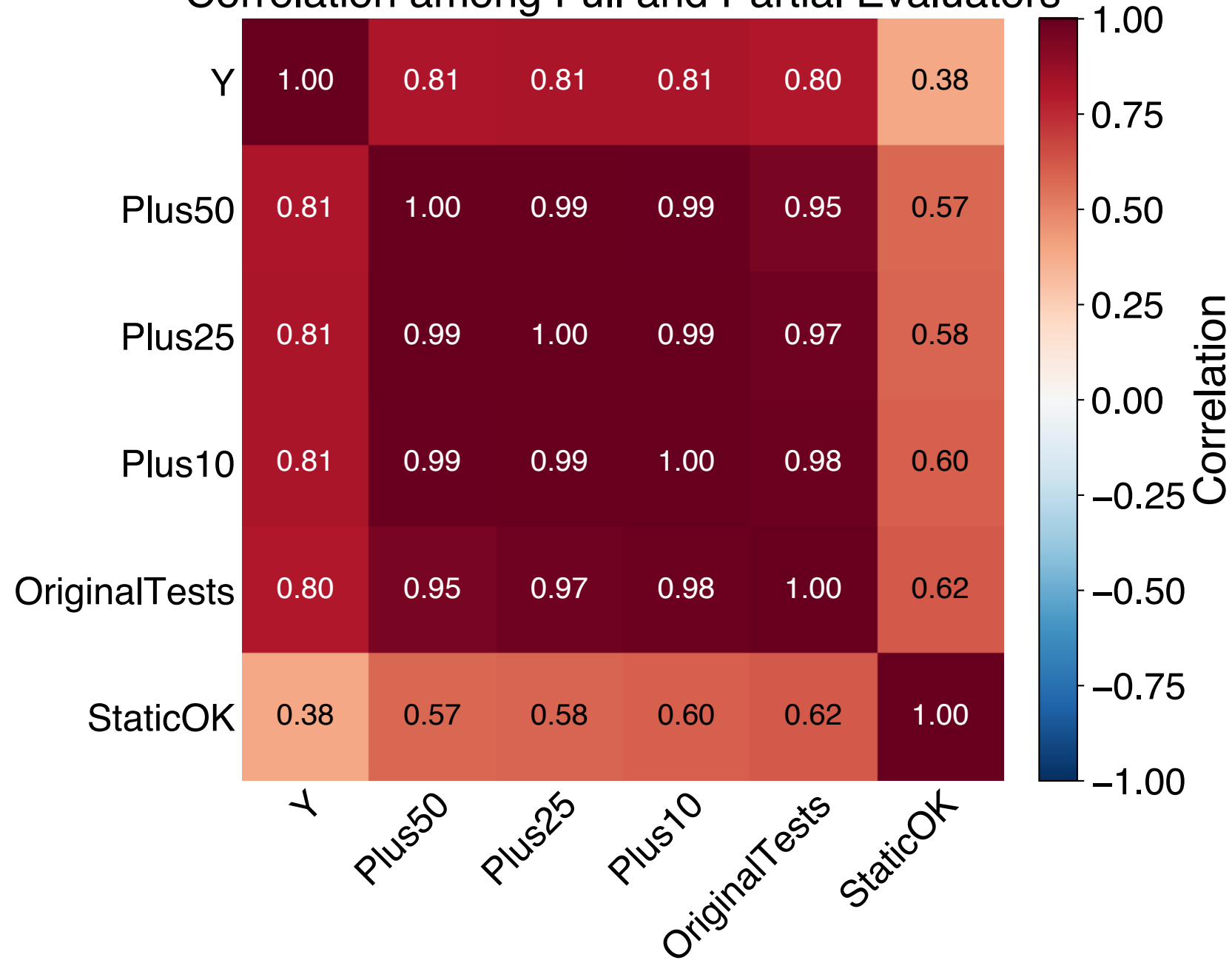
Correlation among Full and Partial Evaluators
