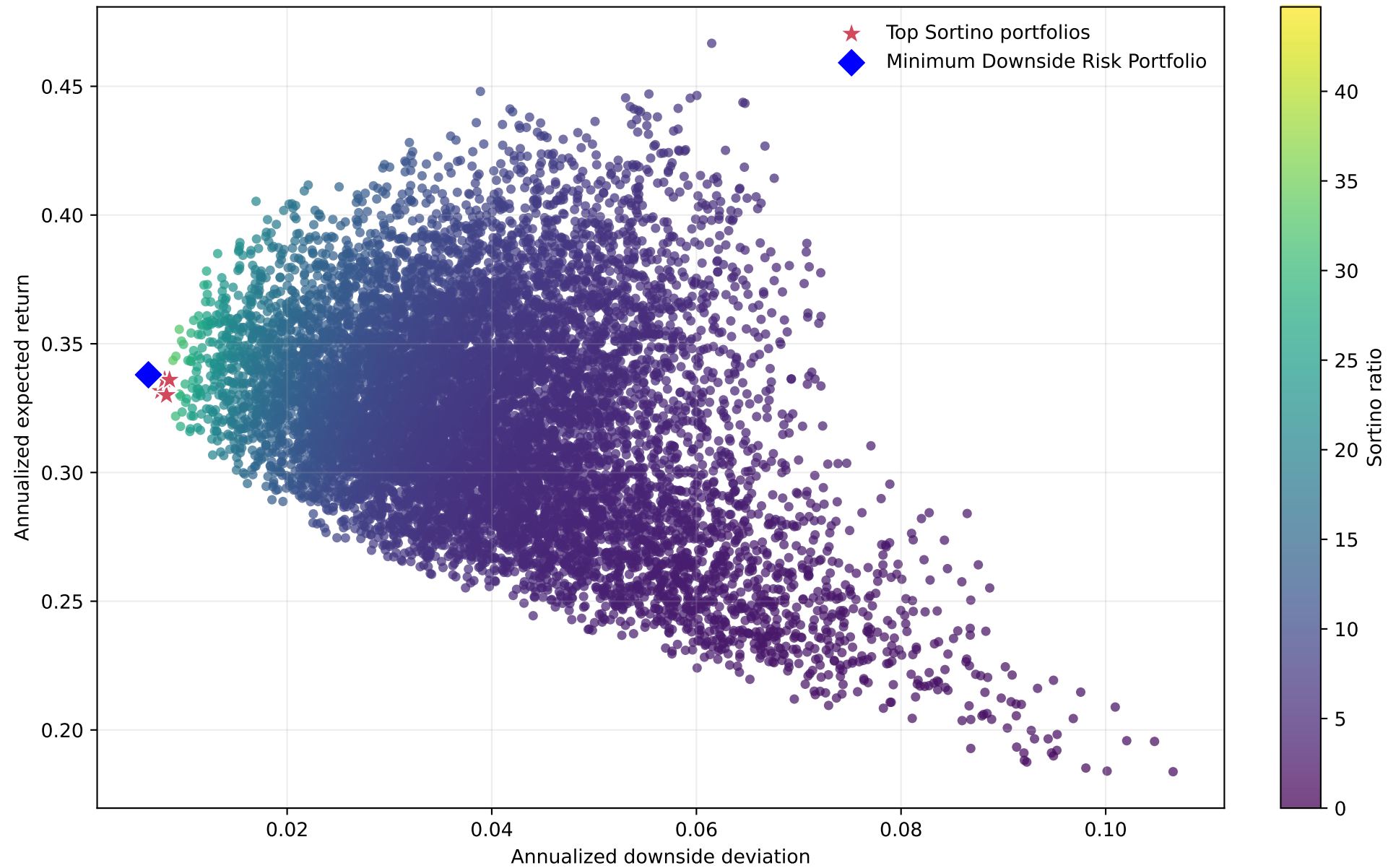
Markowitz Portfolio Simulation
