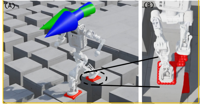
Fig. 3. Foot-mounted height scan to compute the illegal-footstep penalty. Each foot casts a small grid of downward rays, and a ray whose hit point lies more than \delta below the foot signals that the foot overhangs a hole or an edge, as on the stepping stones shown.
