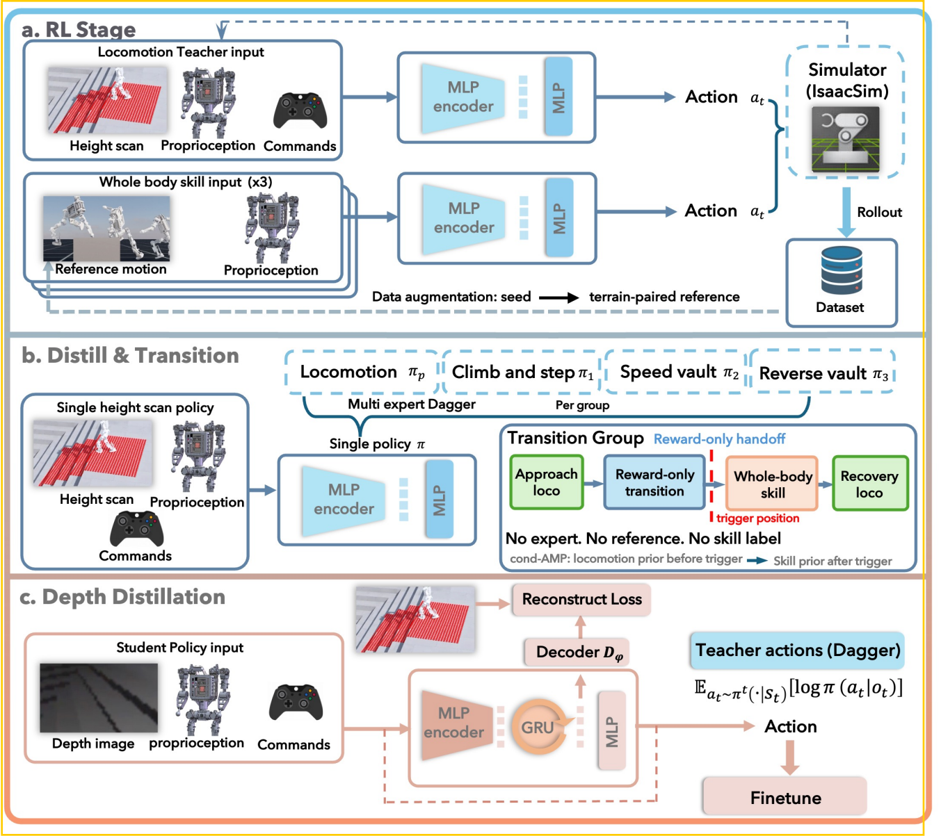
Fig. 2. Overview of Light-LoCo-Parkour. (a) RL stage: using privileged information, we train one perceptive-locomotion teacher and one teacher for each whole-body skill, while data augmentation expands each seed motion into terrain-paired references. (b) Distill & transition: multi-expert Dagger distills the locomotion and skill teachers into a single height-scan policy: a reward-only transition group then fine-tunes the policy to hand off between locomotion and whole-body skills without an expert, reference, or skill label, while the AMP prior switches from locomotion to skill at the trigger position. (c) Depth distillation: the resulting height-scan policy is distilled into a recurrent depth policy using onboard-style depth, proprioception, and velocity commands, with teacher-action supervision, auxiliary height-scan reconstruction, and a final fine-tune.
