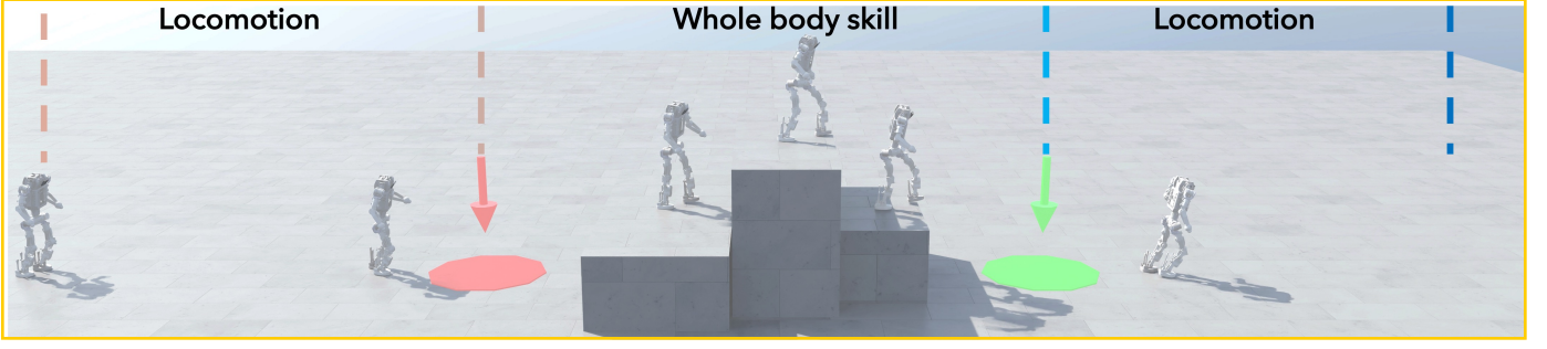
Fig. 6 Transition group. The robot is reset across all three regions, namely the locomotion terrain, the whole-body-skill zone, and the far side of the obstacle, so every phase of a crossing is trained. The conditional motion prior switches from the locomotion AMP to the skill AMP once the robot passes the trigger position.
