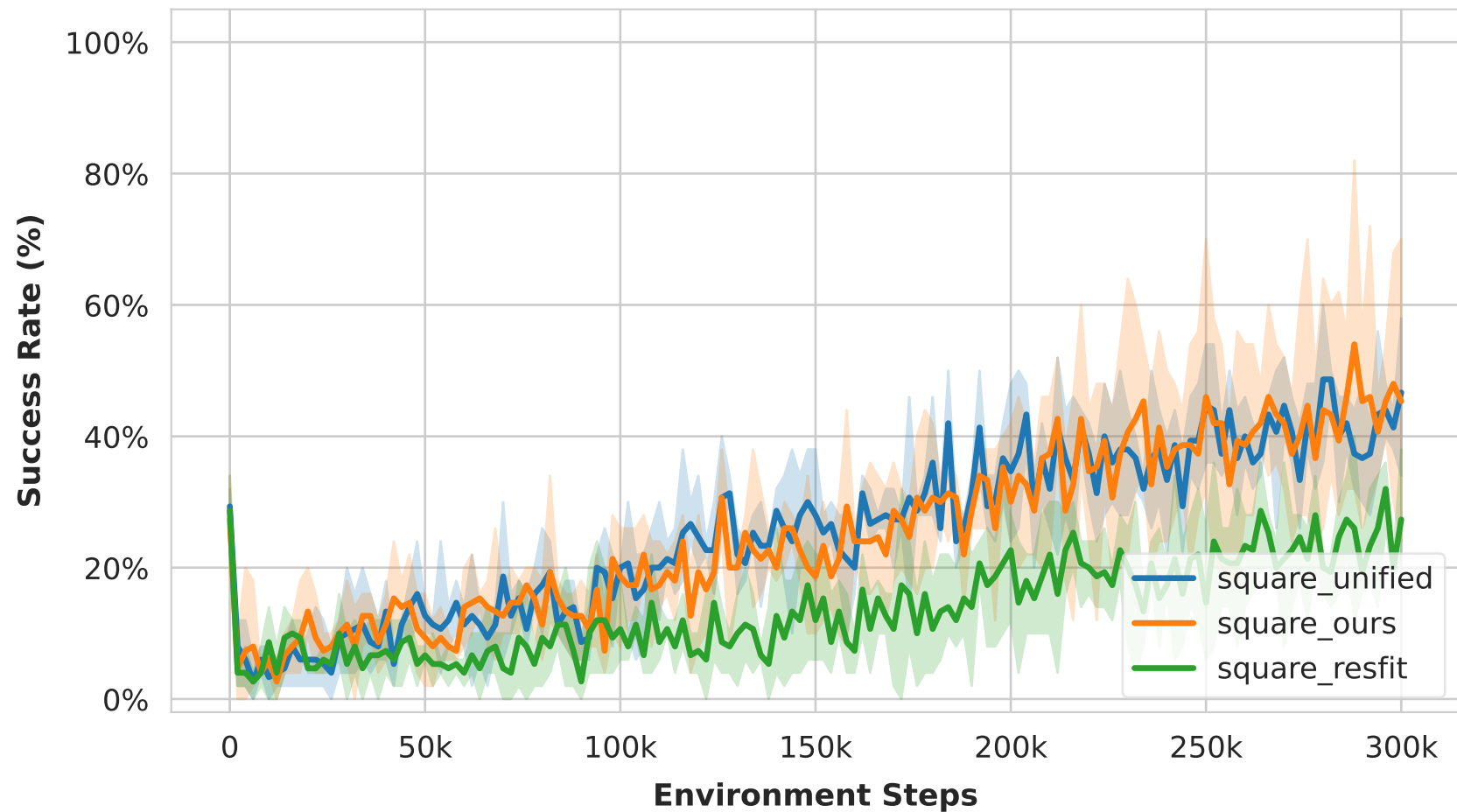
Robosuite Square: Evaluation Success Rate (3 Seeds, Mean & Min-Max Range)
