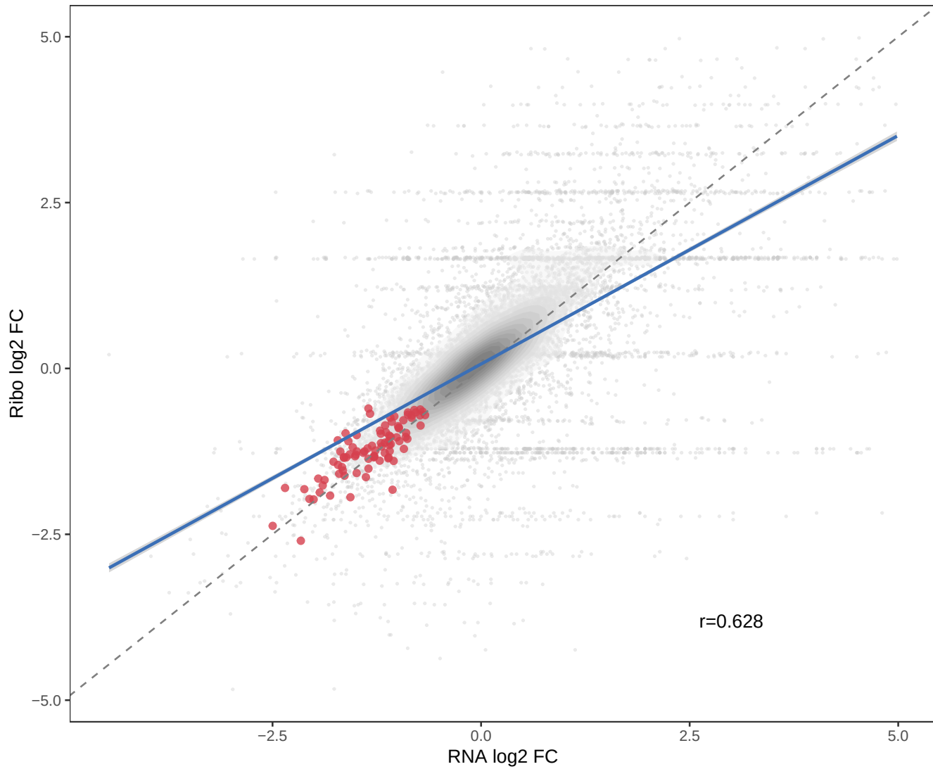
RNA vs Ribo: Scatter Density
