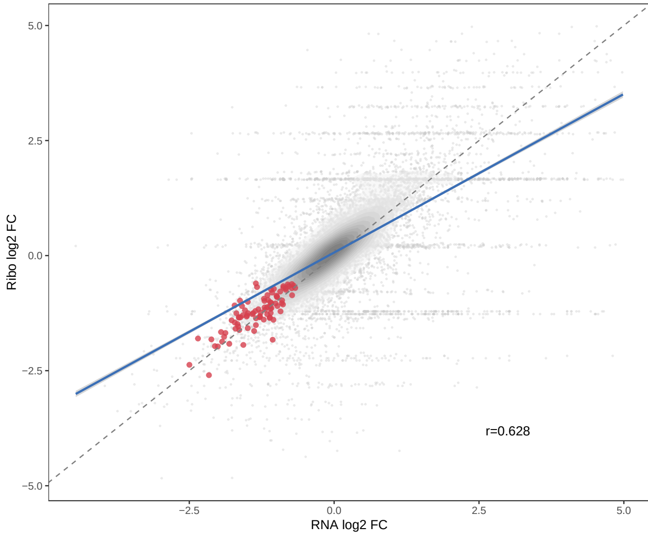
RNA vs Ribo Scatter Density (Template)
