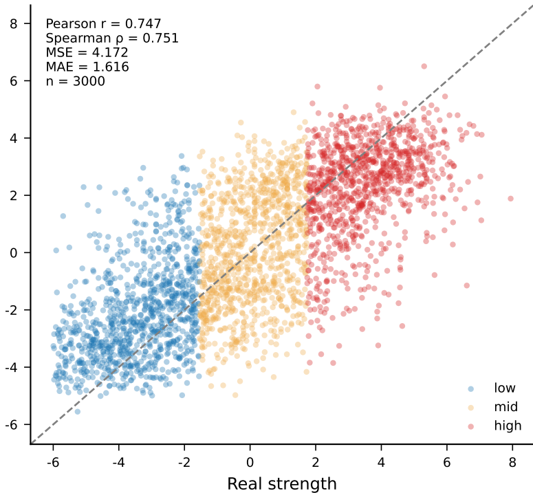
Predictor performance on E. coli test set
