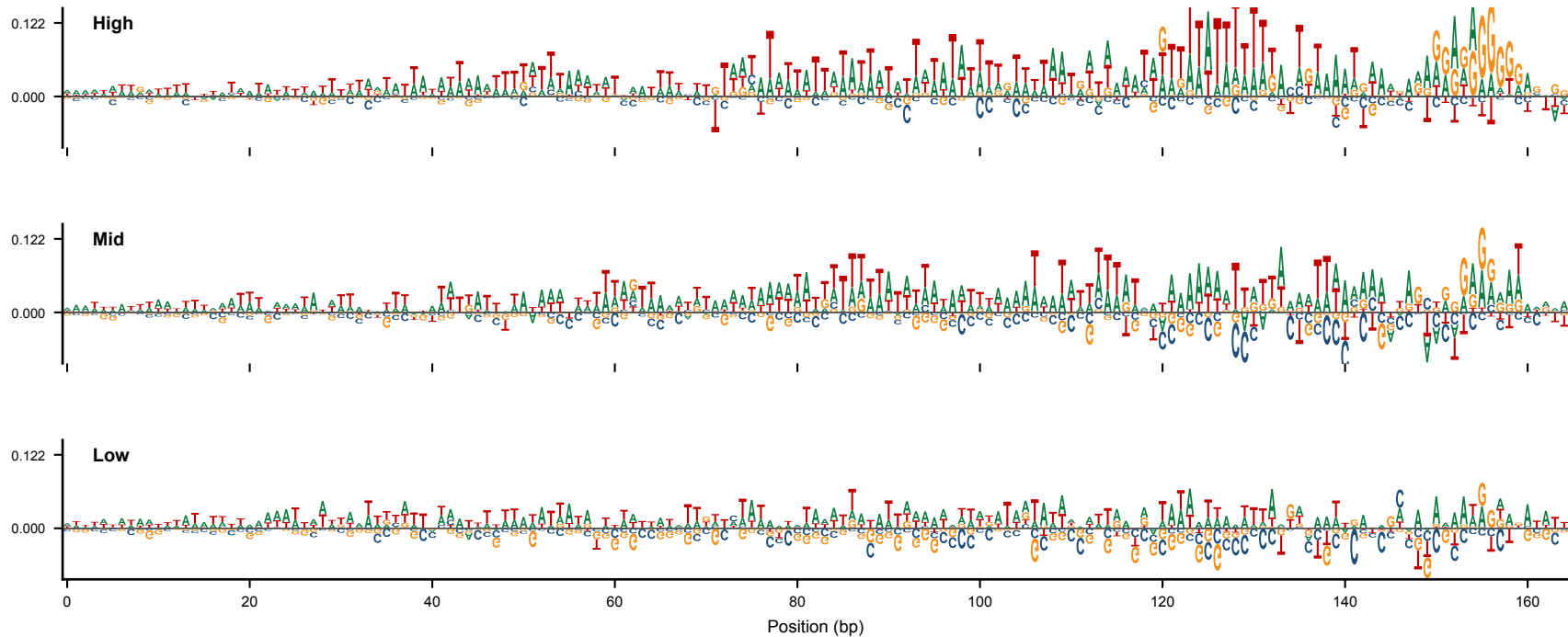
Mean ISM Importance Across Promoter Strength Levels
