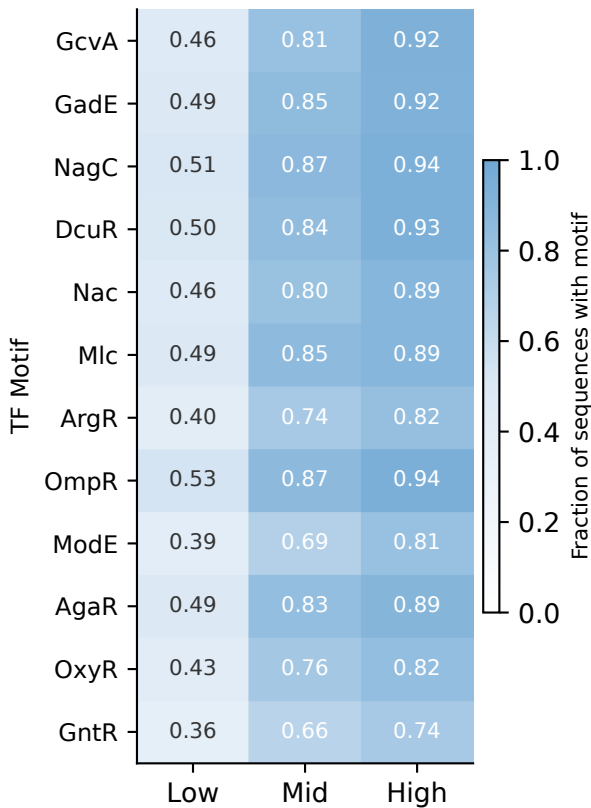
TFBS Enrichment Heatmap (Top 12 by cross-condition variance)
