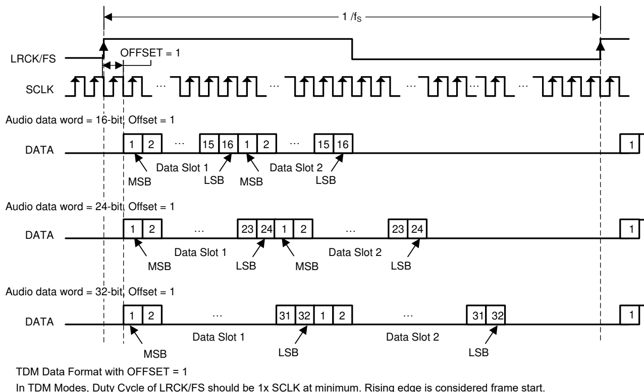
Figure 6-7. TDM 2 Audio Data Format
