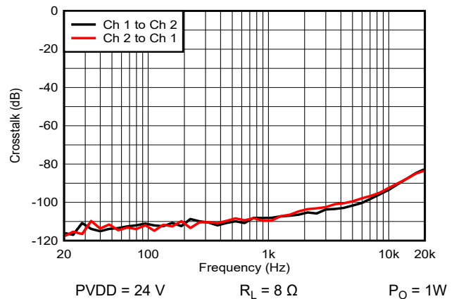
Figure 5-35. Crosstalk
