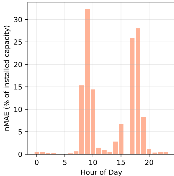
Normalized MAE by Hour
