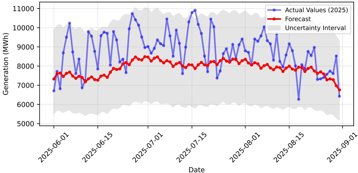
Summer Comparison of Forecast vs Actual PV Generation (Daily Averages)
