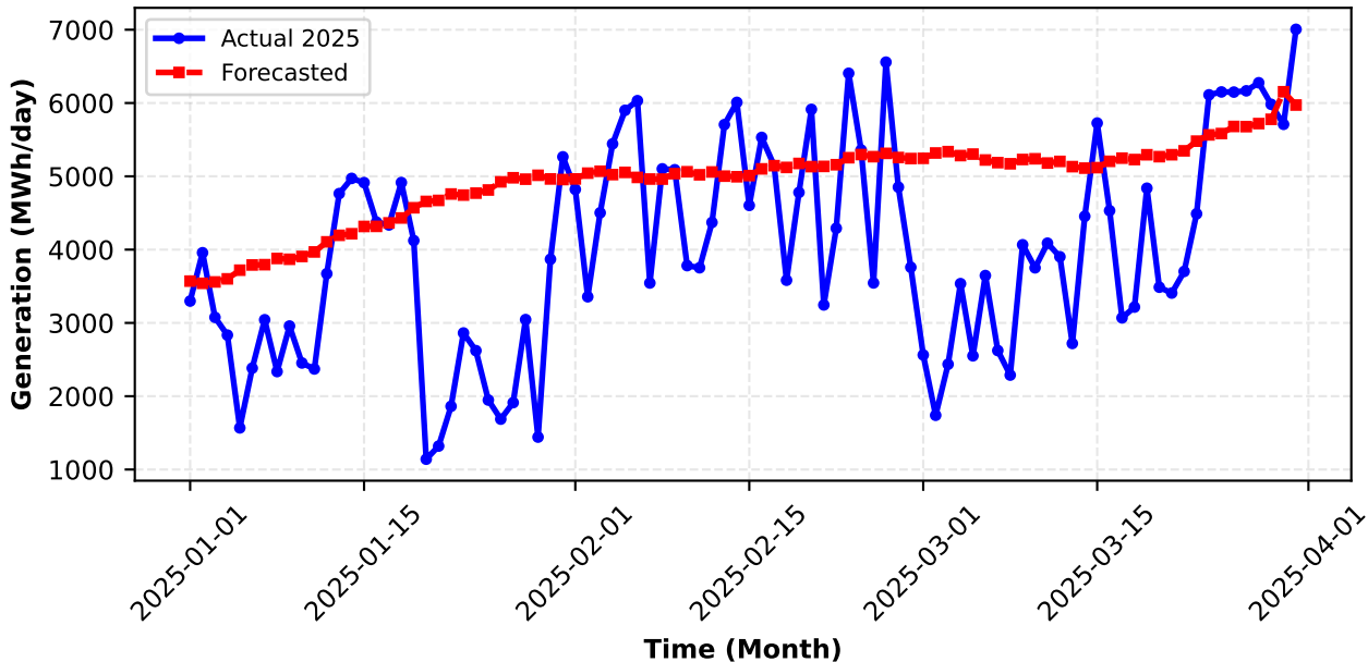
Winter Forecasted vs Actual PV Generation (Daily Average)
