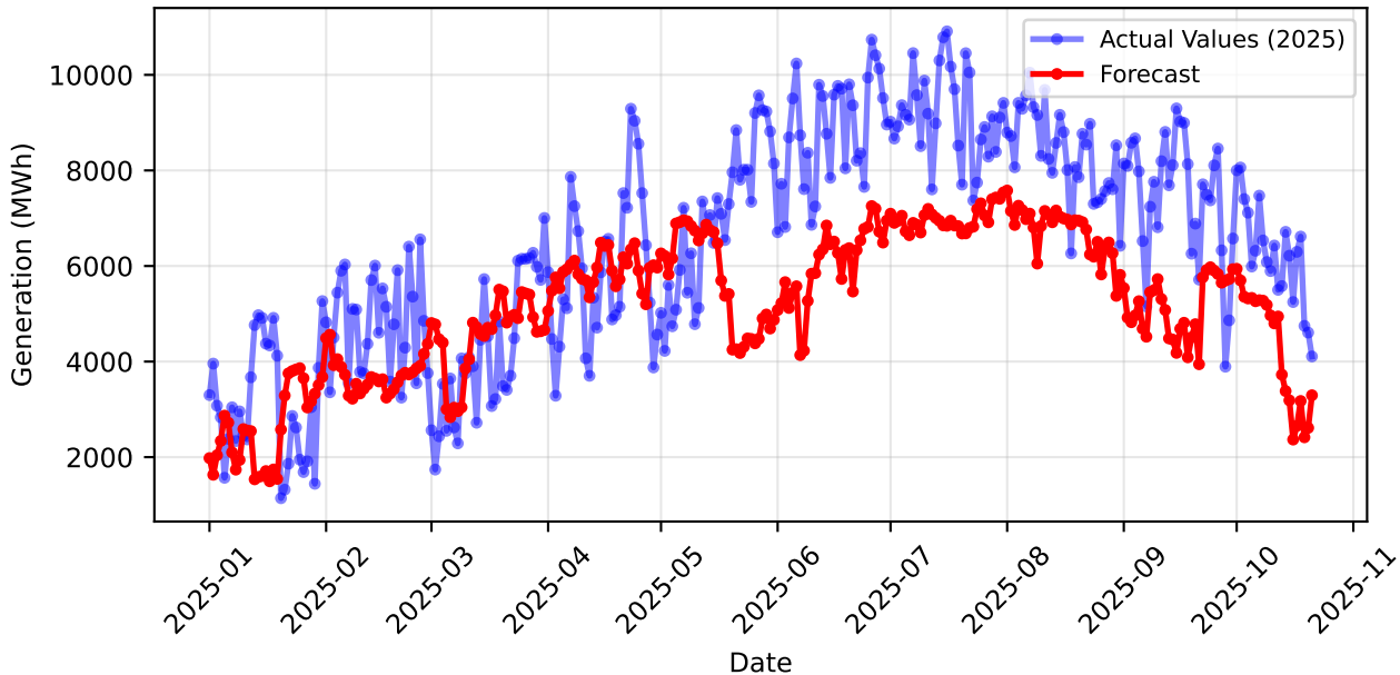
Year-long Comparison of Forecast vs Actual PV Generation (Daily Averages)
