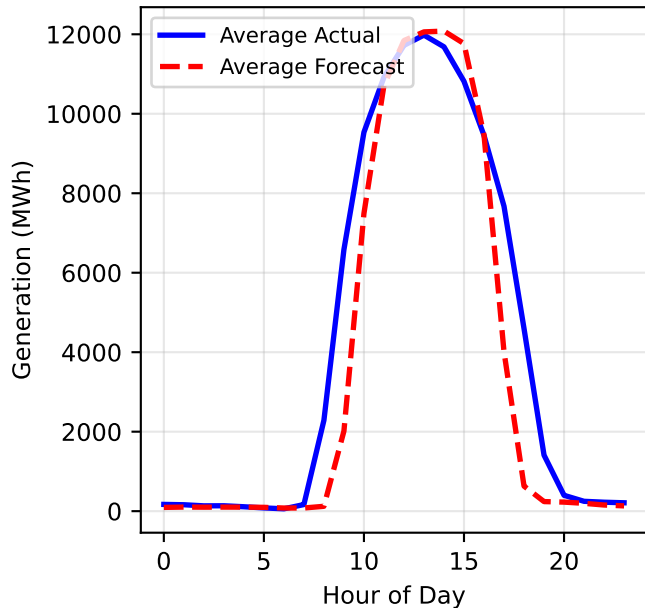
Average Daily Generation Profile (XGBoost)
