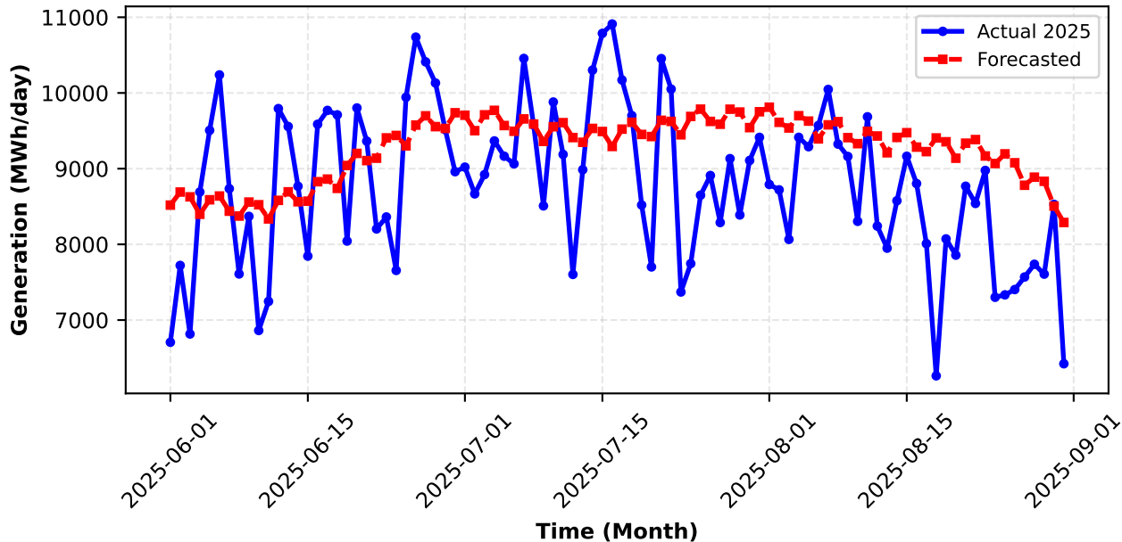
Summer Forecasted vs Actual PV Generation (Daily Average)
