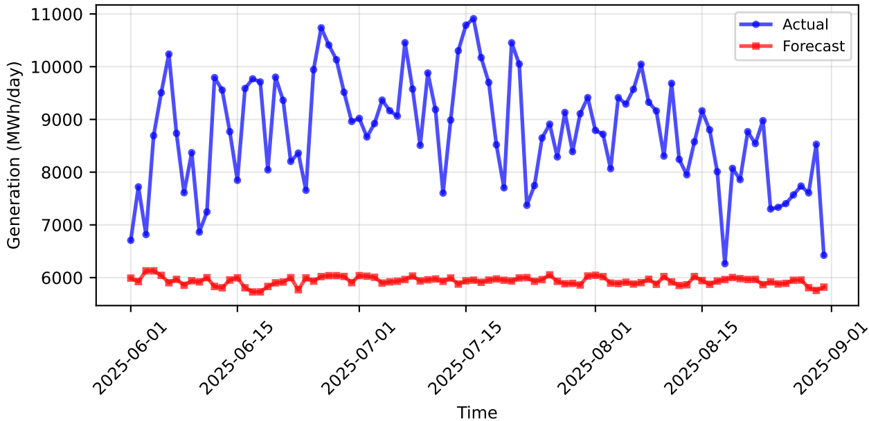
Summer Actual vs Forecast PV Generation (Daily Average)
