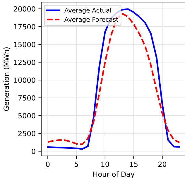
Average Daily Generation Profile
