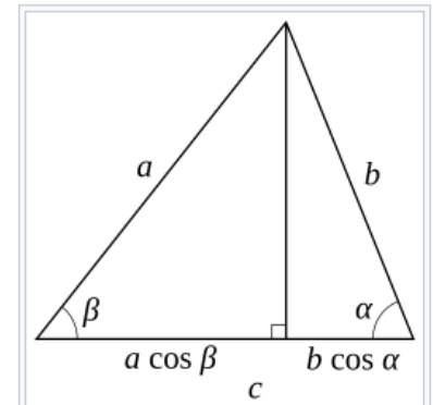
Fig. 5 – An acute triangle with perpendicular
