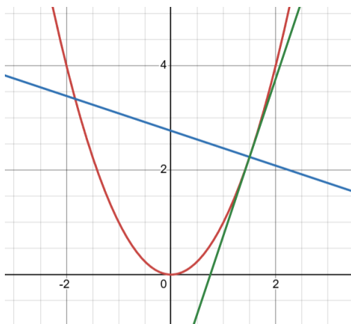
Image of the graph with the tangent and normal added in.
