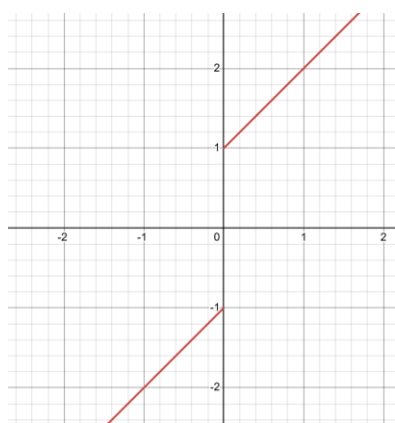
Image: Graph of f(x)
