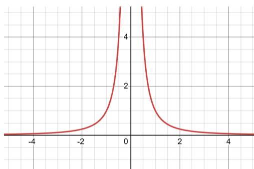
Image: Graph of y = \frac{1}{x^2} .
