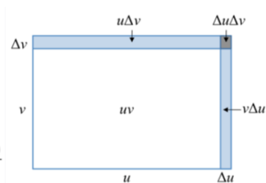
Geometric illustration of a proof of the product rule [1]
