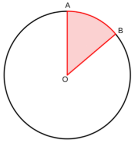
Image of a sector of a circle.
