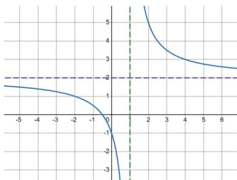
Image: Graph of y = \frac{3}{x-1} + 2
