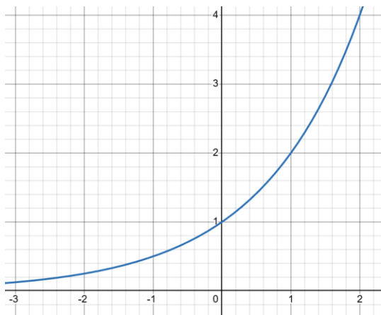
Image: Graph of y = 2^x
