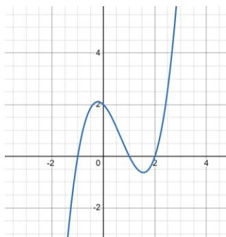
Image: Graph of y = (x - 1)(x + 1)(x - 2)
