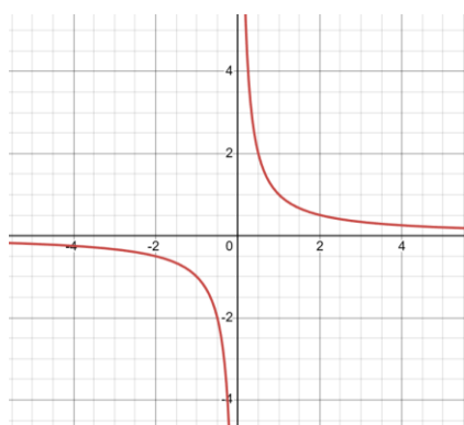
Image: Graph of y = \frac{1}{x} .
