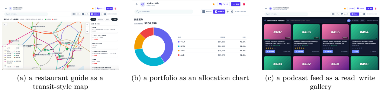
Figure 1: Three of the nine agent-authored custom views in the studied deployment (two collection views and one feed view): a restaurant collection rendered as a transit-style map (a); a portfolio whose host-computed valuations (§4) drive an allocation chart (b); and an ingested podcast feed turned into a read-write gallery (c), where the owner’s rating, notes, and resume position are layered on top of episode metadata. Each is a self-contained HTML file the host serves in a sandboxed, capability-scoped iframe; the owner described each in natural language and never saw the generated markup.
