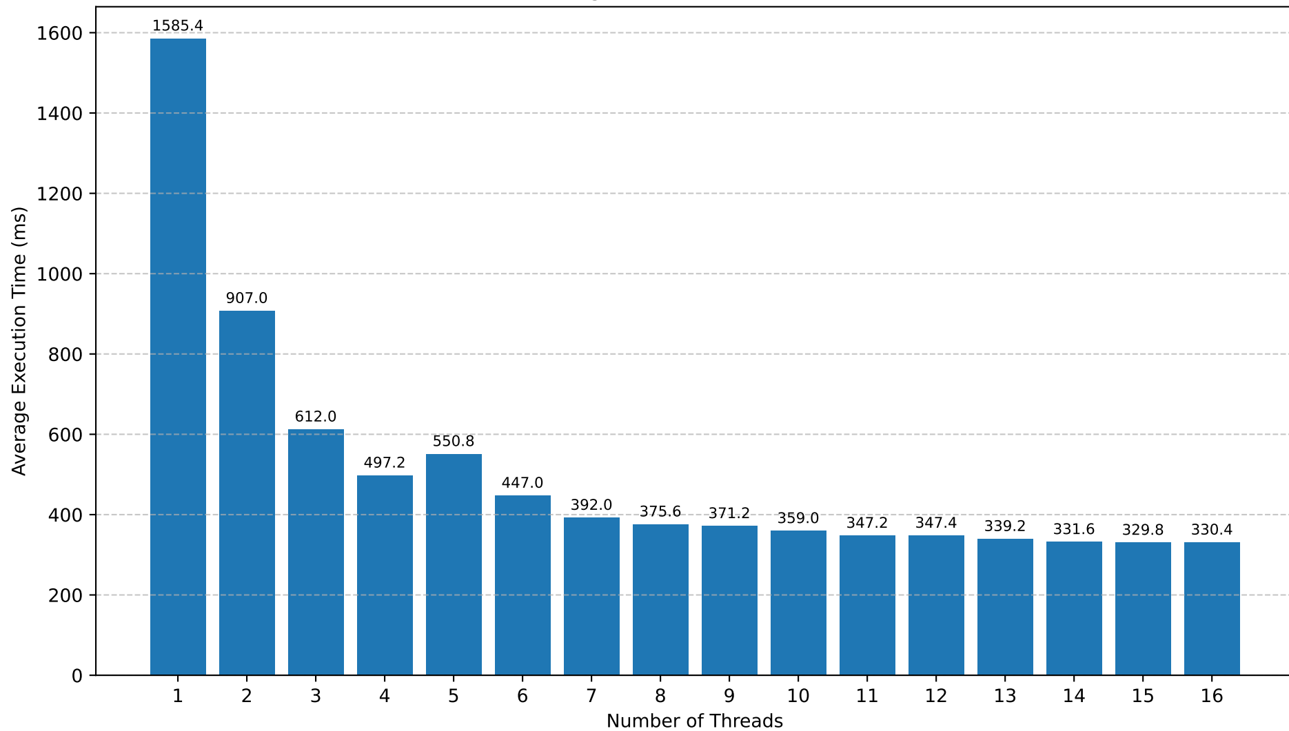
DSGLogBenchmark Performance
