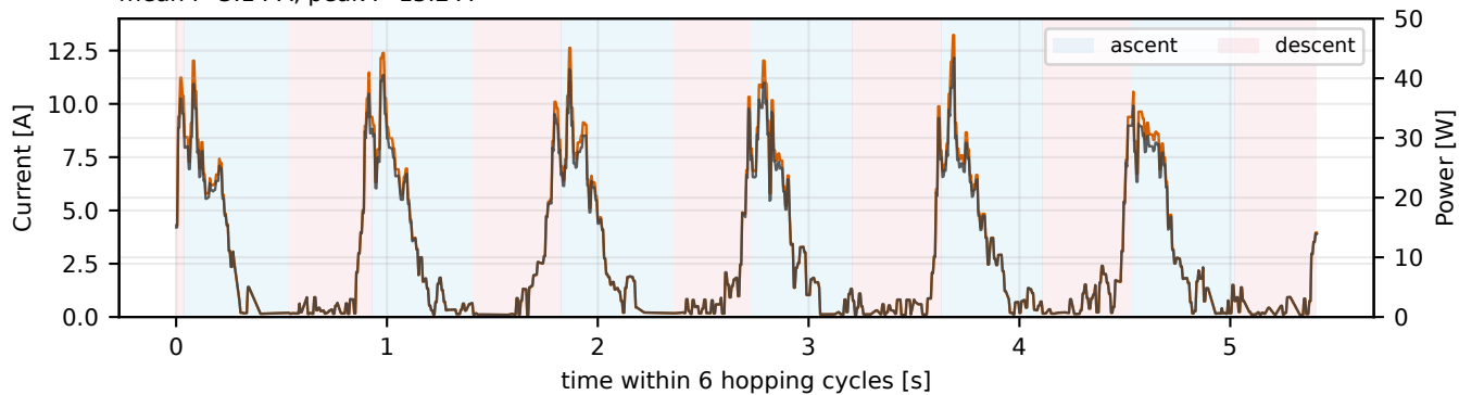
mean I=3.14 A, peak I=13.2 A
