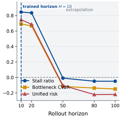
(a) Rollout-depth validity
