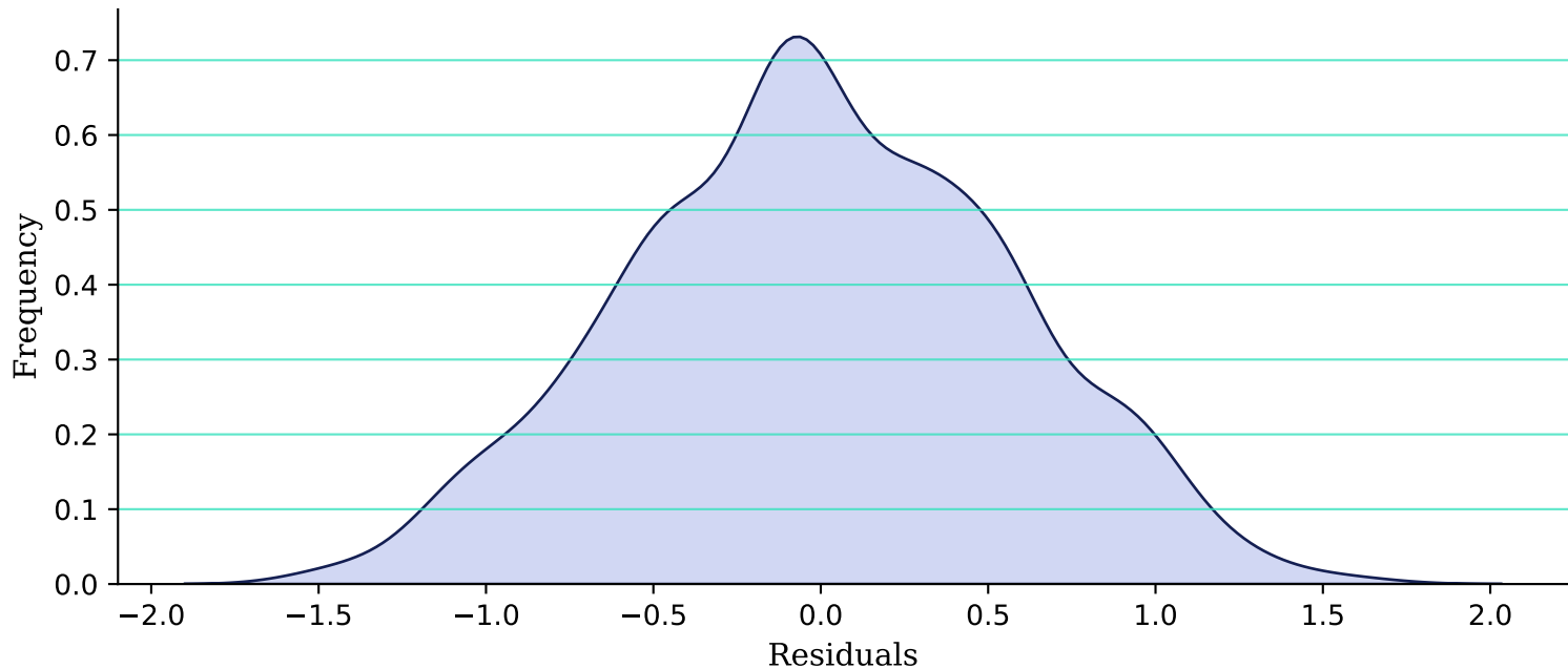
Distribution of Residuals (ANOVA Model)
