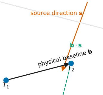
geometric delay
