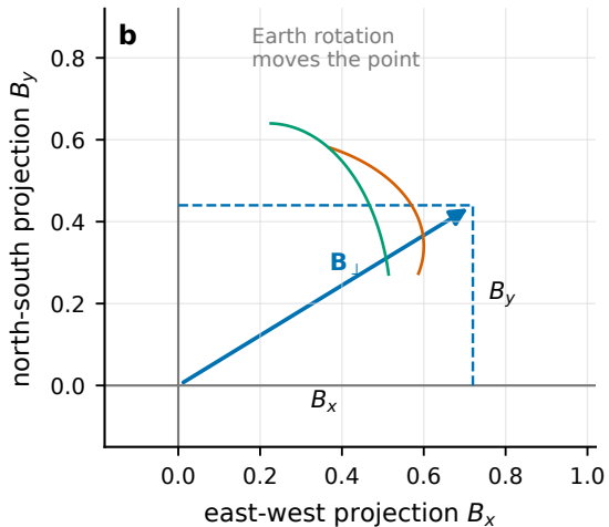
projected baseline on sky
