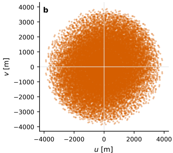
60 telescopes / 1770 baselines
