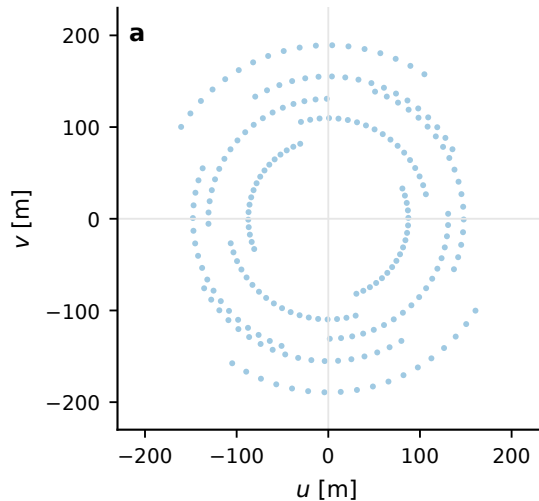
4 telescopes / 6 baselines
