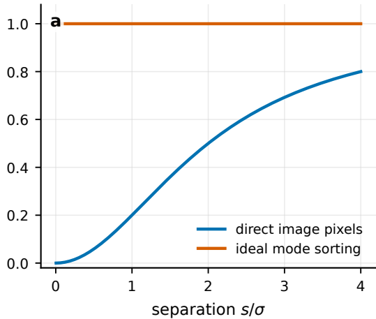
relative Fisher information
