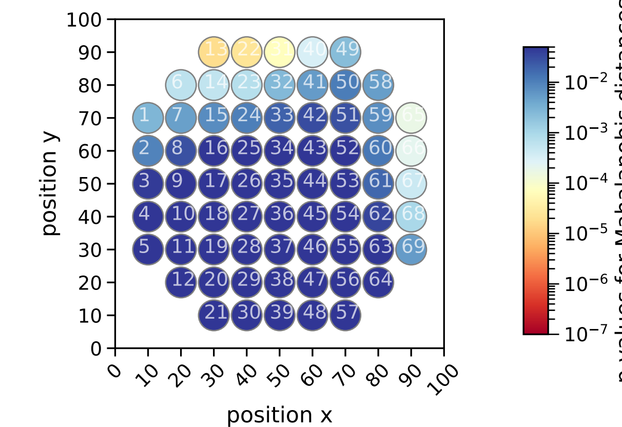
"distance" from new FeCrNiCoV data to hardness dataset
