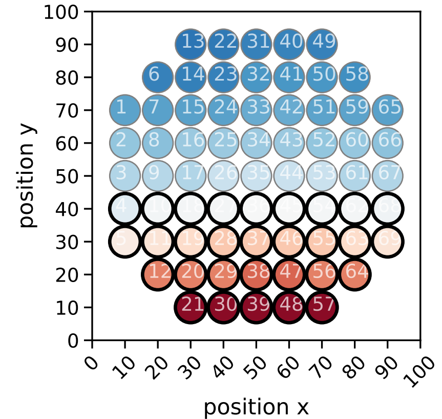
NiCrCoVFe scored relative to corrosion literature
