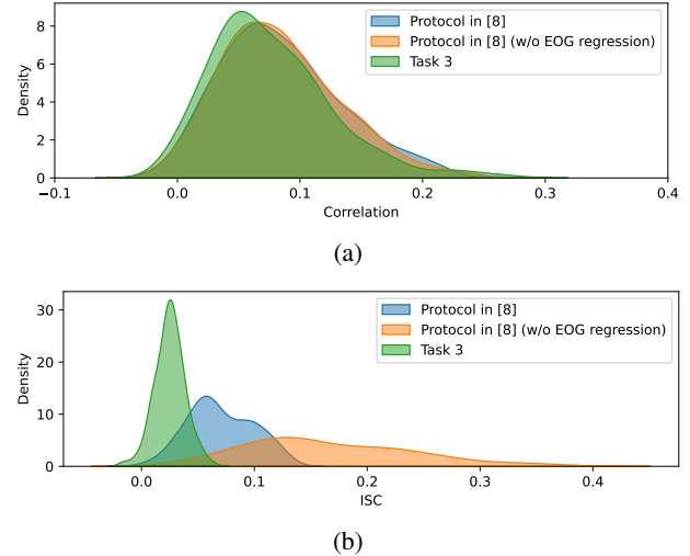
Fig. 8: Distributions of (a) stimulus-response correlations and (b) inter-subject correlations across participants for 45-second segments under the free-viewing and gaze-fixation protocols. The values represent the sum of the first two components. For comparison, results obtained from EEG without EOG regression are also included. For the gaze-fixation condition, only Task 3 (attend, central) is shown. Curves are Gaussian kernel density estimates computed from approximately 500 45-second segments (pooled across participants) for (a), and 100 45-second segments for (b). The bandwidth was selected automatically by Scott’s rule, the default of seaborn’s kdeplot .
