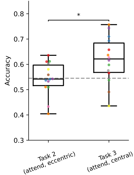
Fig. 9: Match-mismatch (MM) decoding accuracy for the attend-eccentric (Task 2) and attend-central (Task 3) conditions on 45-second test segments, obtained with CCA spatial filters estimated separately within each task. This differs from Figure 4, where the filters are estimated from the combined data of all three tasks. Individual participant accuracies are shown as colored dots, with statistical outliers circled (identified by the Tukey 1.5 \times \text{IQR} rule; outliers were retained in all Wilcoxon signed-rank tests). Box plots display the median and interquartile range, with whiskers extending to extreme values. The dashed line indicates the significance bound for above-chance performance, defined as the 97.5th percentile of the circular permutation null distribution recomputed for the present per-condition decoders (1400 permutations). The asterisk denotes a significant difference between tasks (Wilcoxon signed-rank test, p = 0.028 , Z = 1.91 , rank-biserial r = 0.58 ). Task 3 accuracy exceeds Task 2 accuracy, confirming that the eccentricity effect persists under within-task filter estimation.
