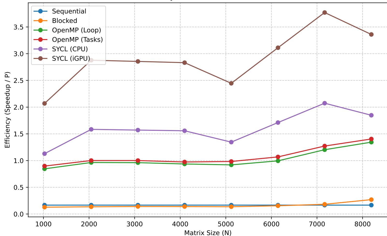
Efficiency vs Matrix Size (P=6 cores)
